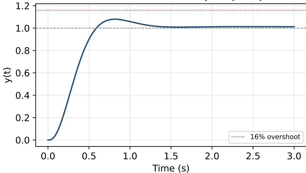
Problem 27: Final closed-loop step response
